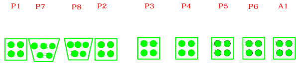
PILE FOUNDATION
